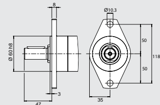
Stainless steel Flange Ordering No. 4430 2357 80
