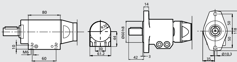
Foot Ordering No. 4430 0178 80
